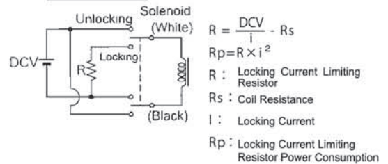
Operation Circuit
